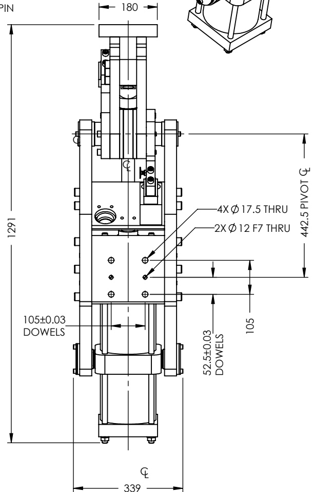
HORIZONTAL MOUNTING DIMENSIONS
