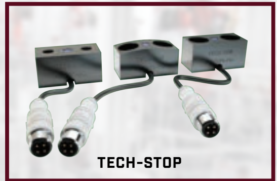
NAAMS Stop Blocks with integrated inductive sensors
