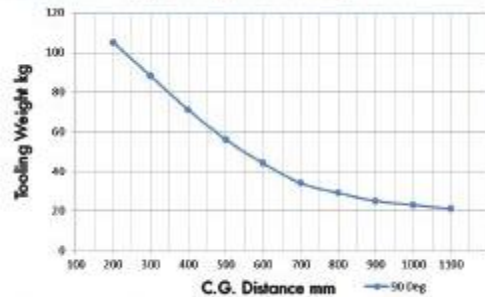
TECH-PIVOT 100 (VERTICAL/HORIZONTAL)
