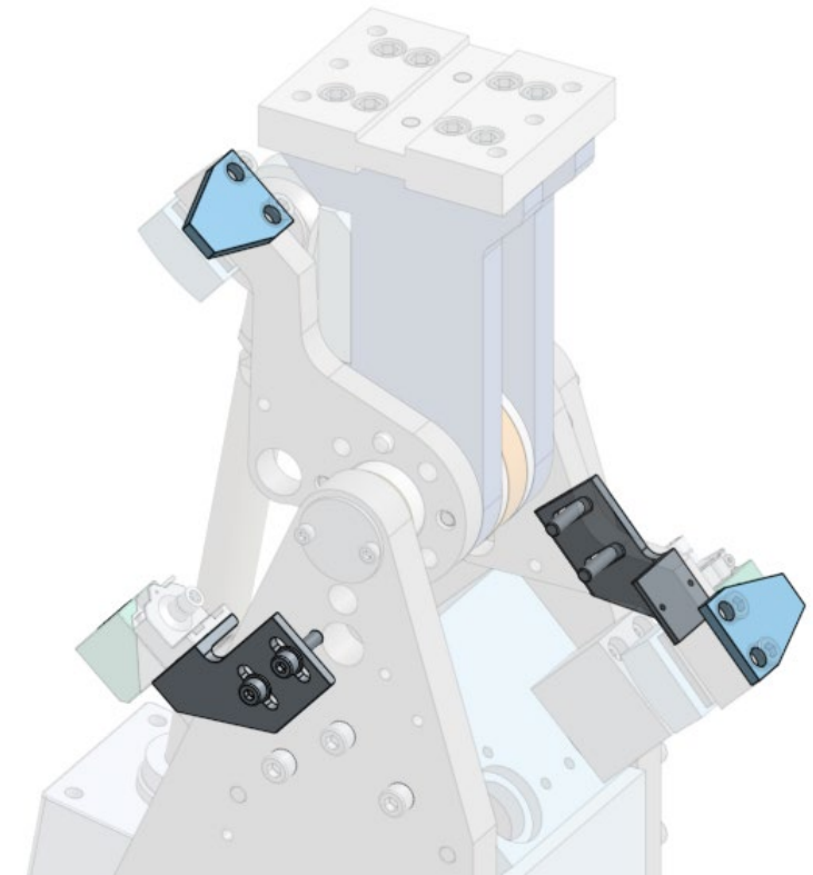
PC , CUBE BRACKET, OUTBOARD EXAMPLE PART NUMBER TR100-H-90-6-1L- PC -A
