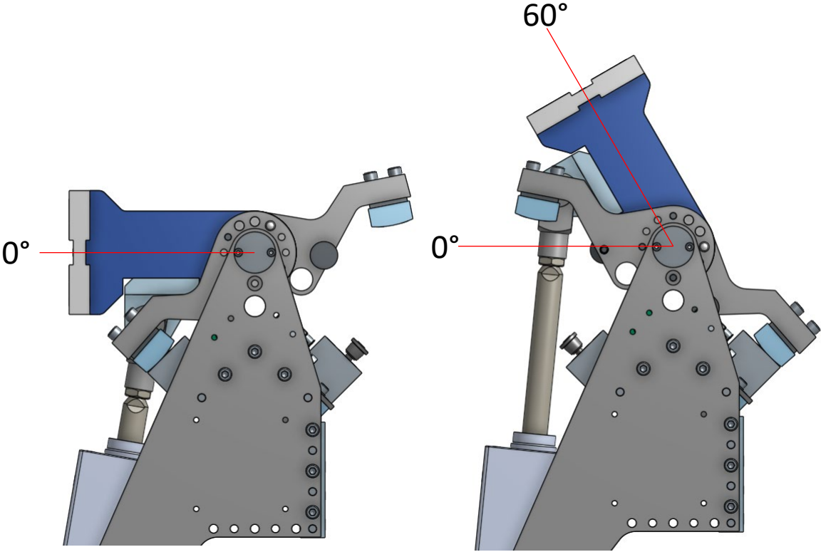
WORK / HOME POSITION (CYL RETRACTED)
