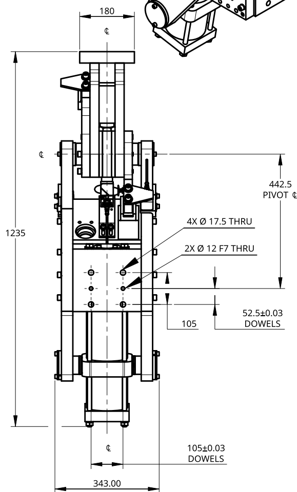
HORIZONTAL MOUNTING DIMENSIONS
