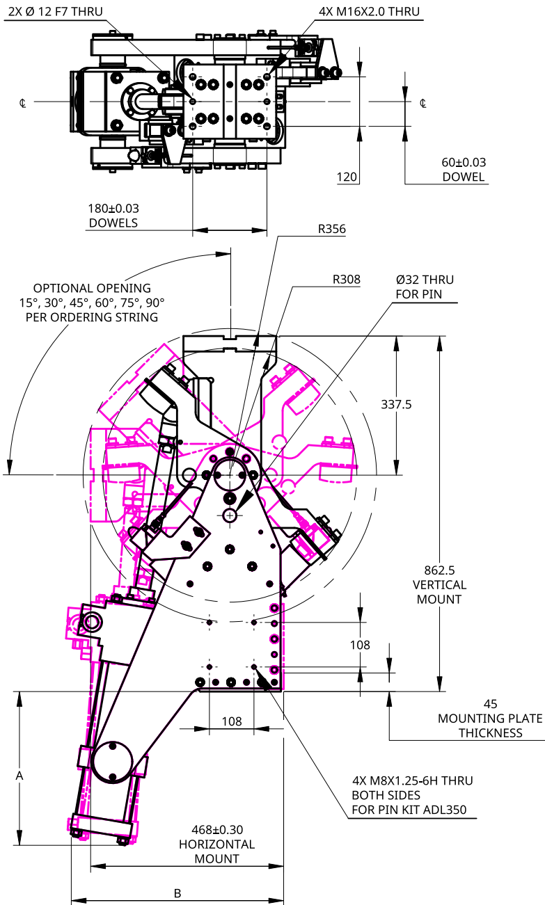
HORIZONTAL MOUNTING DIMENSIONS
